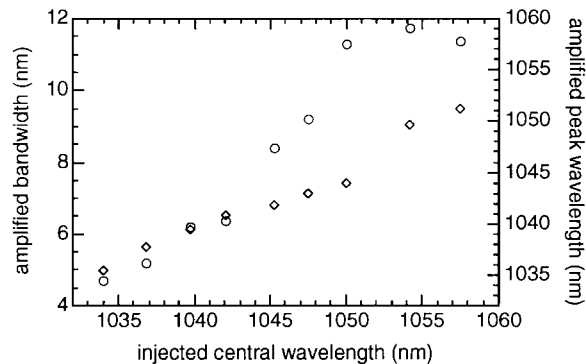
Fig. 3. Amplified bandwidth (circles) and amplified peak wavelength (diamonds) as a function of the injection pulses' central wavelength.
